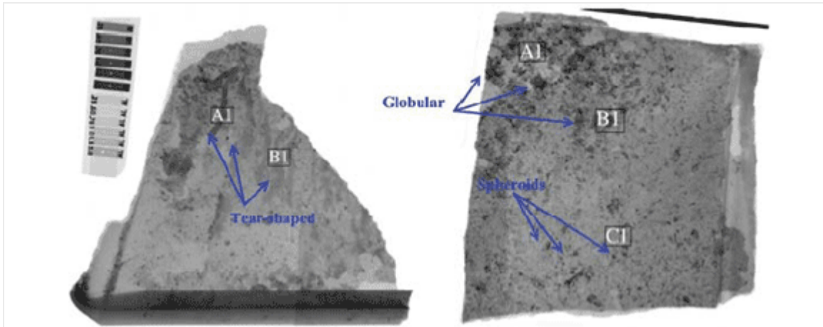
Figure 16. The types of deposition patterns observed on radiographic images of LH RCC panel 8 pieces.
